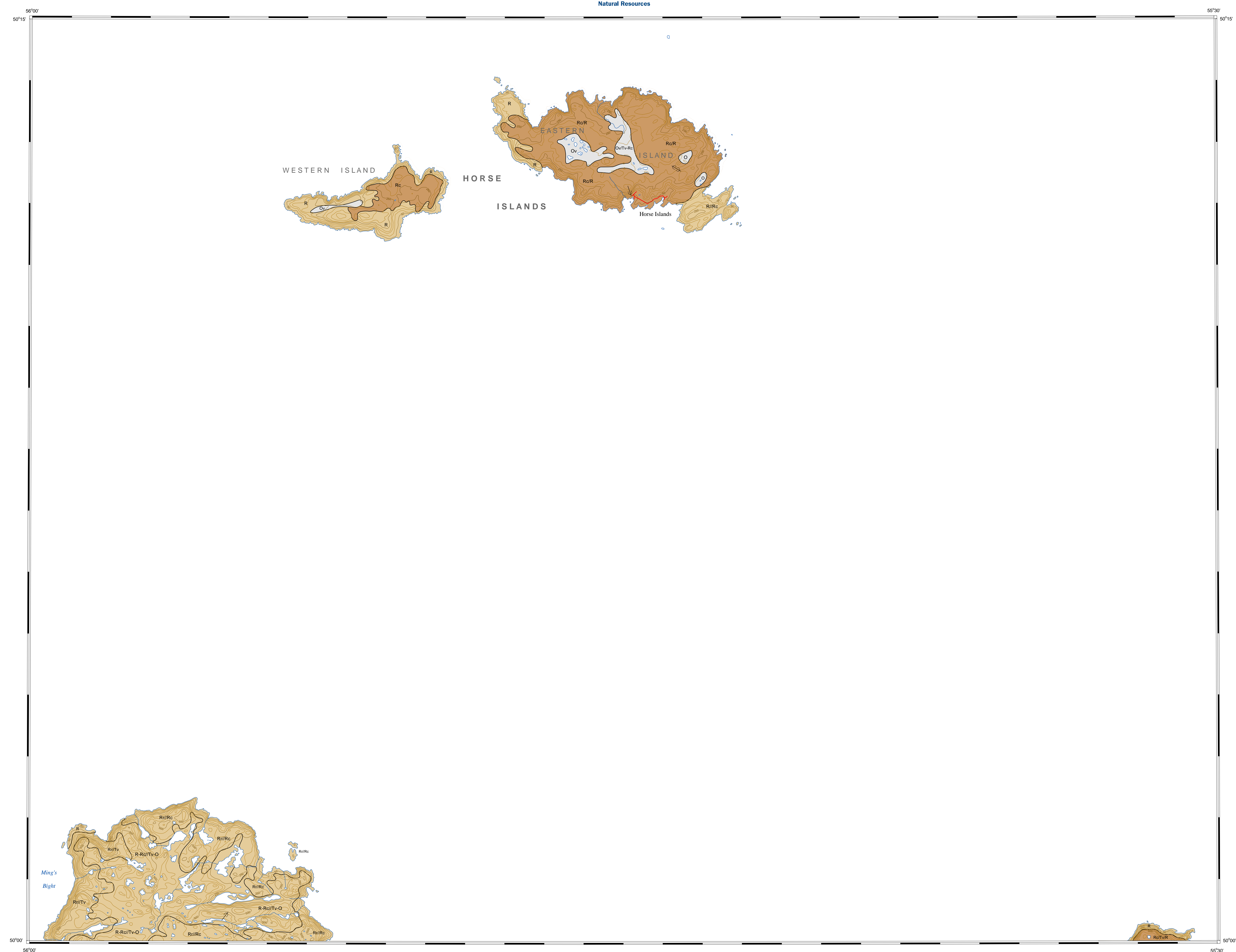
MAP 2011-04 HORSE ISLANDS NEWFOUNDLAND AND LABRADOR
