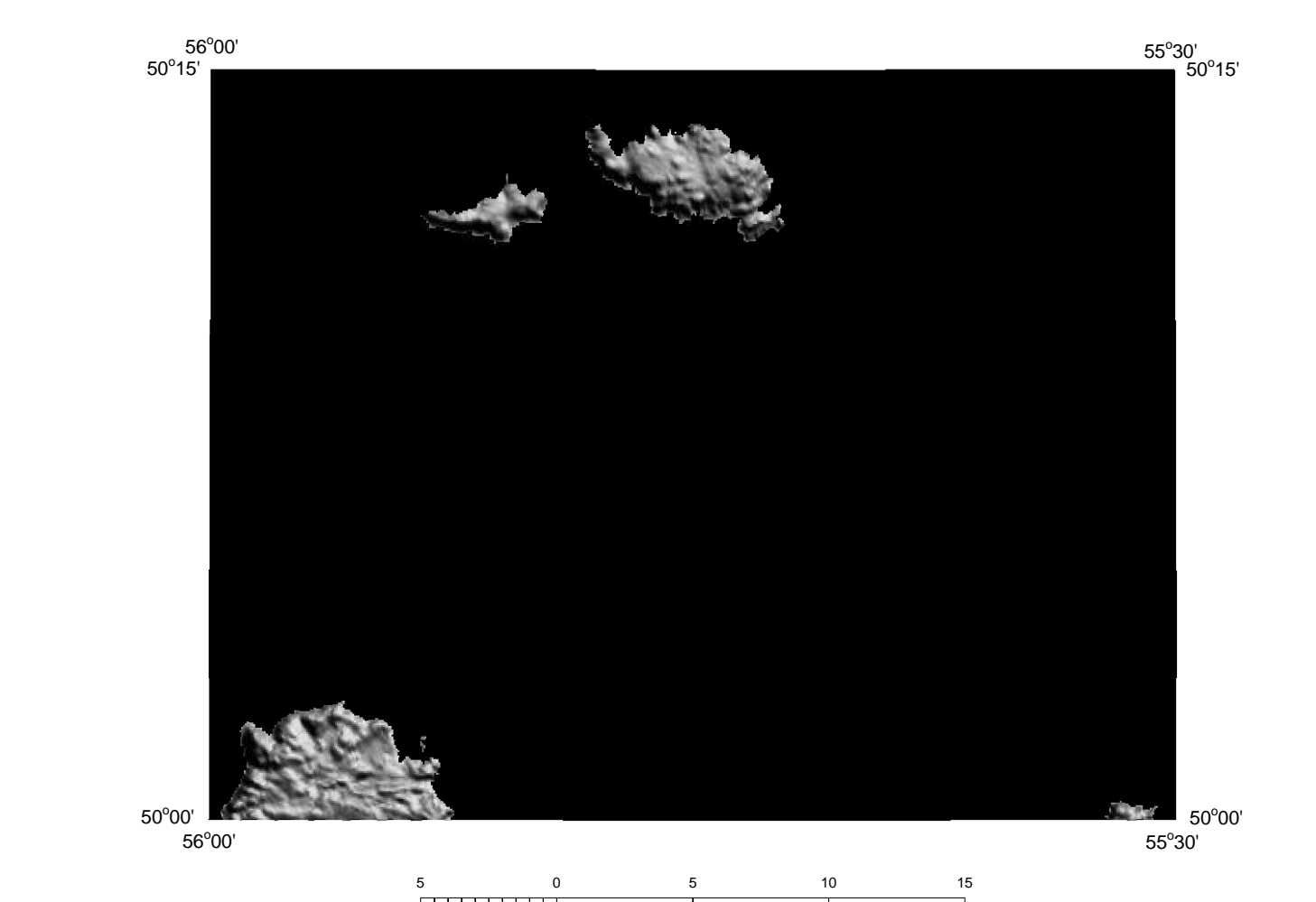
Digital Elevation Model (DEM) from Shuttle Radar Topography Mission (SRTM) data of the Horse Islands map area (shaded from the north-east). The image provides surface information not readily illustrated on the surficial map. Terrain variability is evident, with areas of bedrock highlighted as rougher textured areas (consistent with surficial map), and areas of thicker till shown as smoother textured areas.
